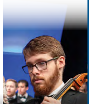
Strings
